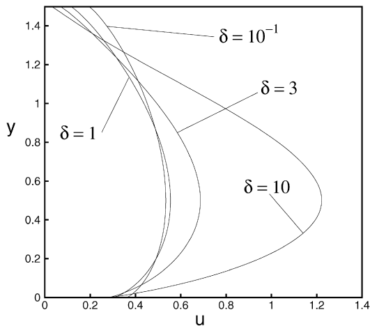
Fig. 6. Velocity profiles for the equilateral triangle along the symmetry axis.
